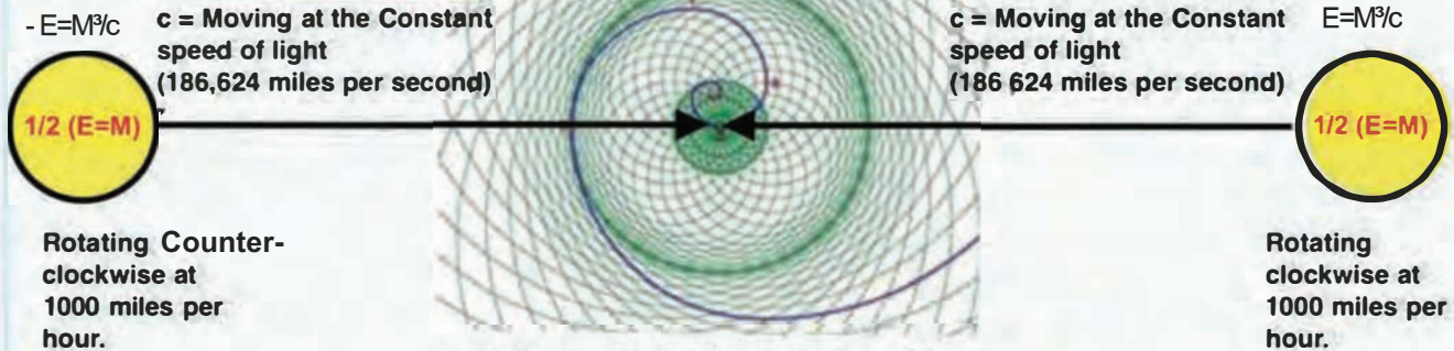
Figure #5 E=Mc^2
